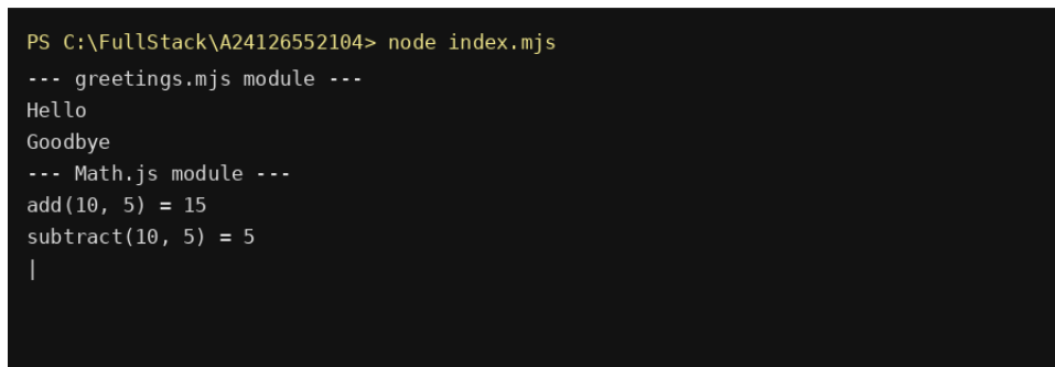
Fig 9.5: Terminal output after running 'node index.mjs', showing exported functions from greetings.mjs and Math.js in action
